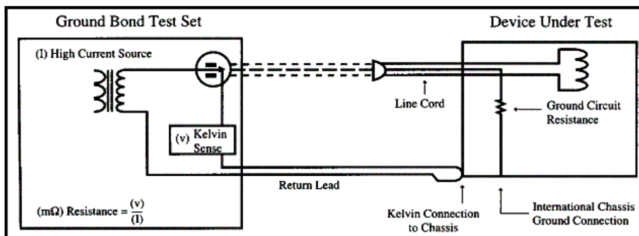
Figur 2: Kredsløbsdiagram for Ground Bond test.
